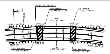
STRUCTURE /ROADWAY RELATIONSHIP
