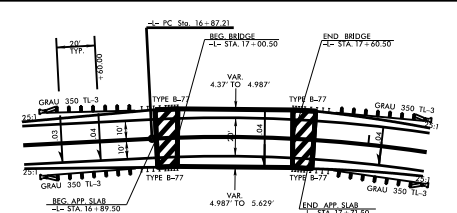
STRUCTURE /ROADWAY RELATIONSHIP
